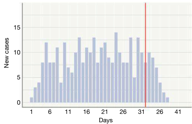
Fig. 5.6 Epidemic curve for a notional outbreak within a single ongoing source. Red line indicates time point where source of infection was removed (e.g. closure of a restaurant).
