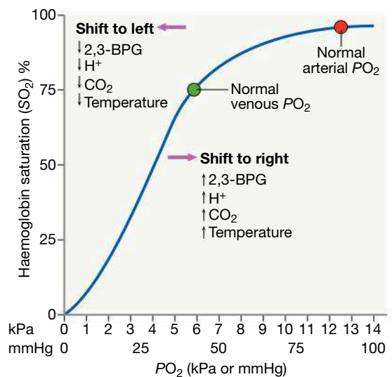
Fig. 25.5 The haemoglobin–oxygen dissociation curve. Factors are listed that shift the curve to the right (more oxygen released from blood) and to the left (less oxygen released) at given \text{PO}_2 . To convert kPa to mmHg, multiply by 7.5. (2,3-BPG = 2,3-bisphosphoglycerate).
